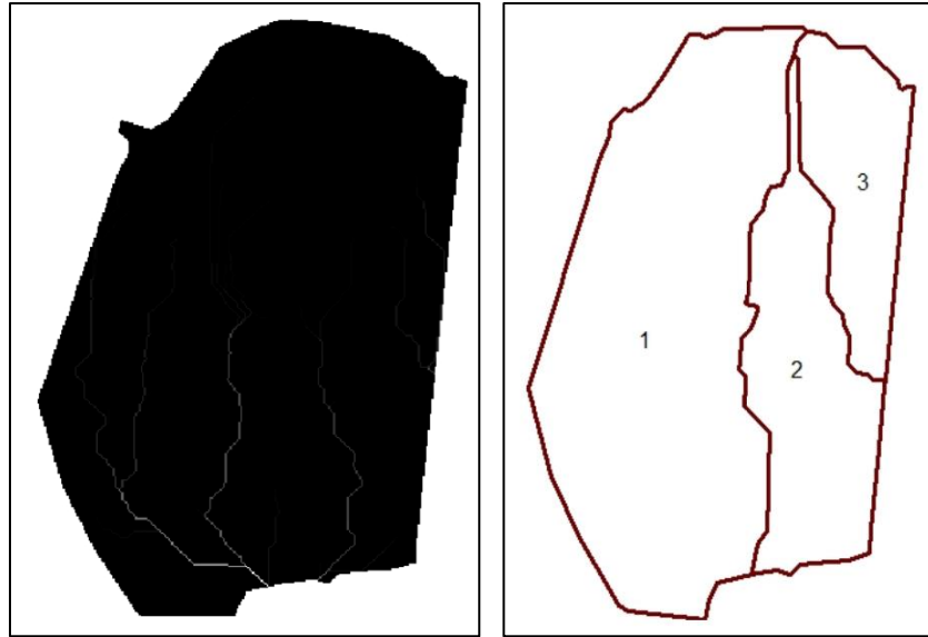
Figure 3-2: Flow accumulation path and sub basins – National Heroes Circle
