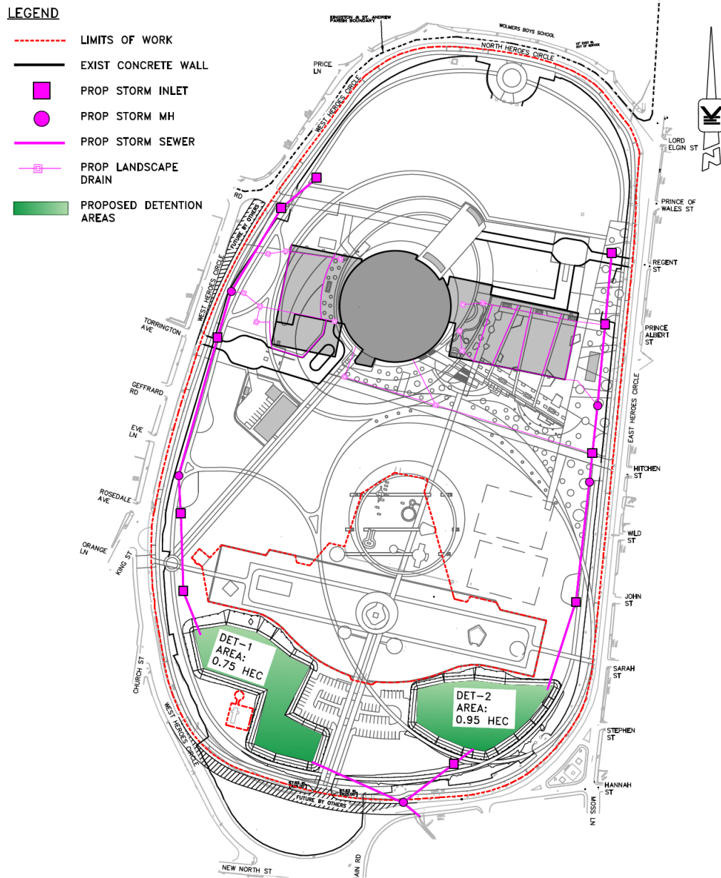
Figure 7-1: Water detention areas and storm sewer plan
